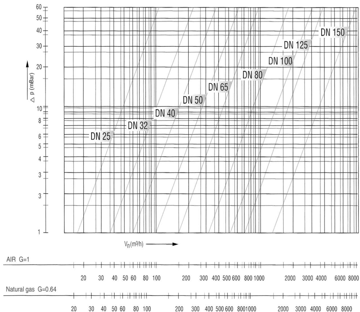
CAPACITY CURVE OF BUTTERFLY VALVES (UP TO 6")
